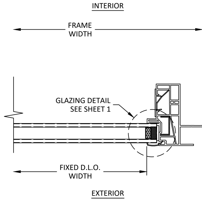
E 4 HORIZONTAL SECTION FIXED JAMB
