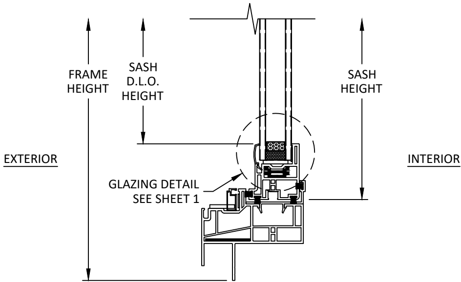
B 3 VERTICAL SECTION SILL
