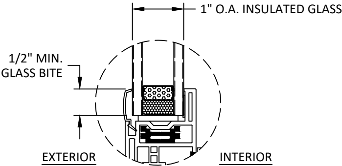
GLAZING DETAIL
