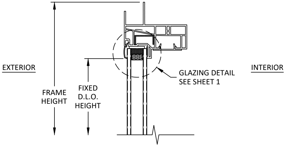
A 3 VERTICAL SECTION HEAD
