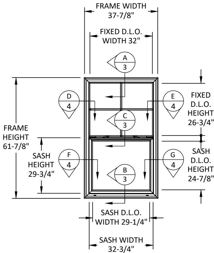
TYPICAL ELEVATION
