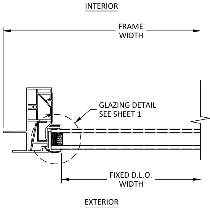
D 4 HORIZONTAL SECTION FIXED JAMB
